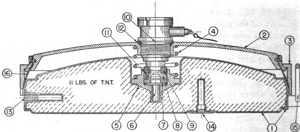
FIGURE 21.—Tellermine—sectional view.
